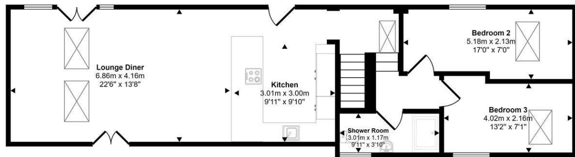
First Floor Approx 74 sq m / 801 sq ft
